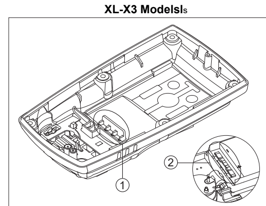
Figure 14. Replacing the Rear Shell
